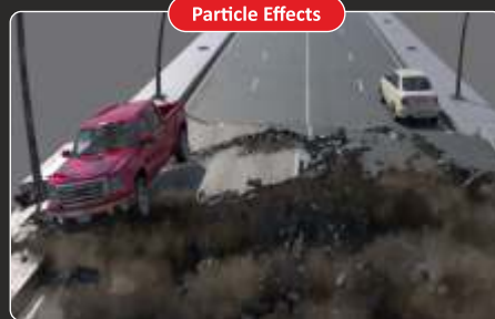
Particle Effects
